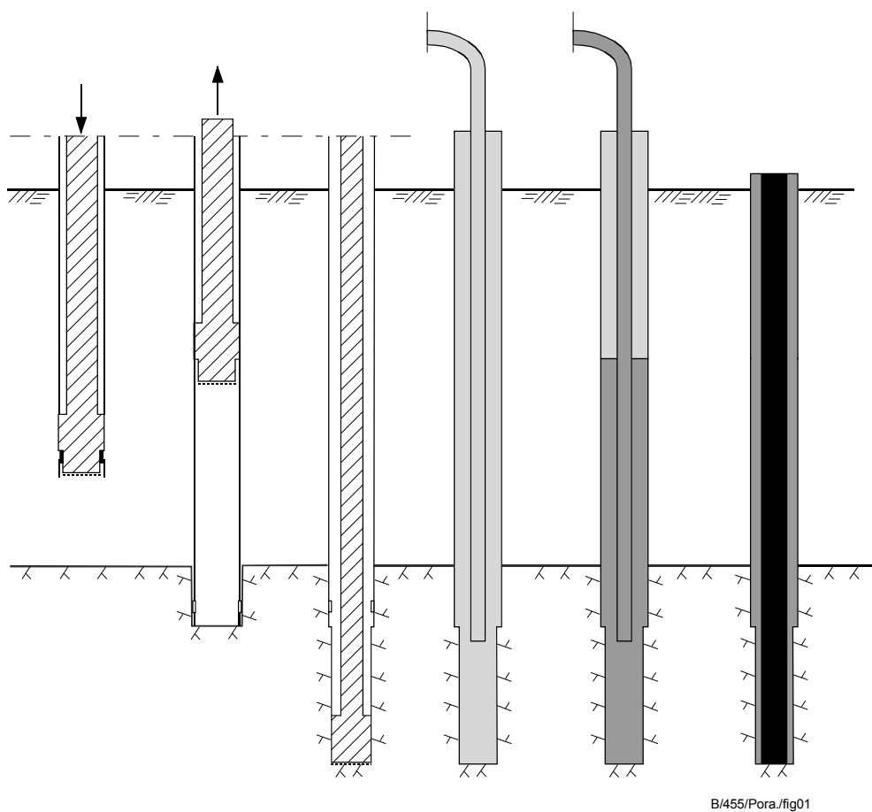
Fig. 1. Installation phases of a steel core pile.
