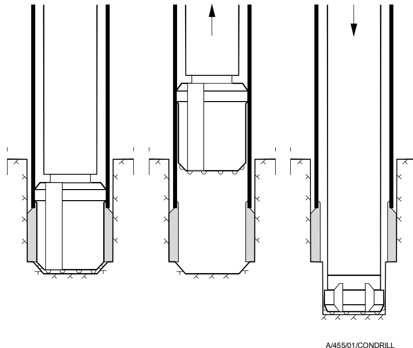
Figure 16. The concentric drilling method
