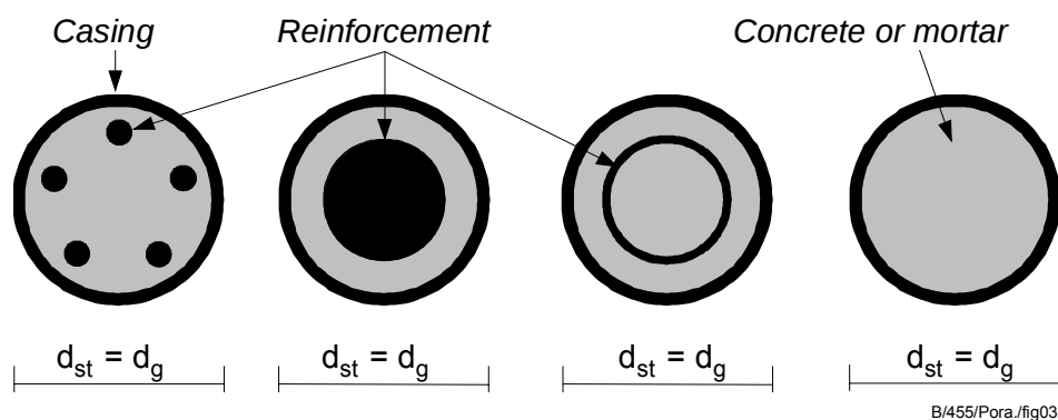
Fig. 3. Reinforcement alternatives for drilled steel pipe piles when the casing becomes part of the pile.
