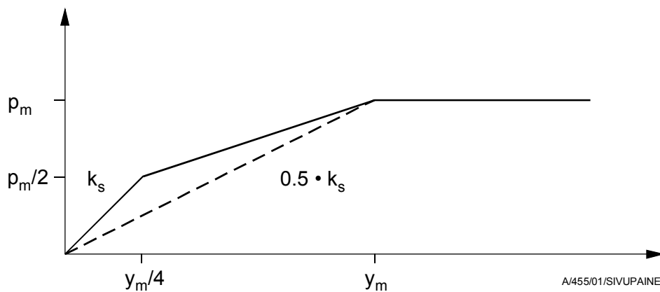
Figure 11. Lateral pressure-pile displacement relation in coarse-grained soil.
