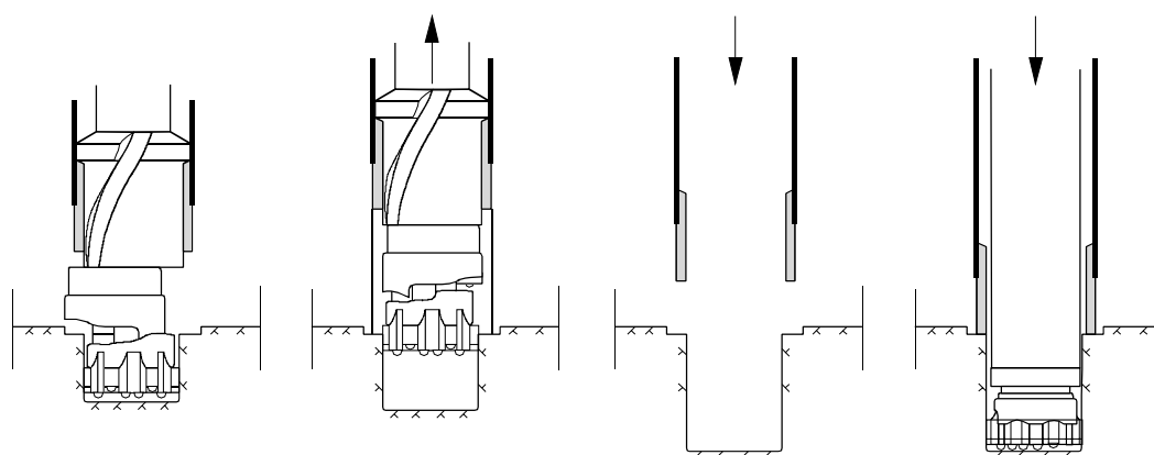
Figure 15 The eccentric drilling method
