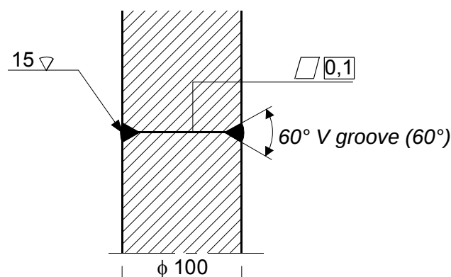
Fig. 9. Example of welding design for solid bar.
